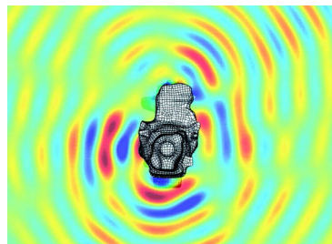
Pressure field generated by a powertrain, whose vibration was calculated by MSC Nastran
