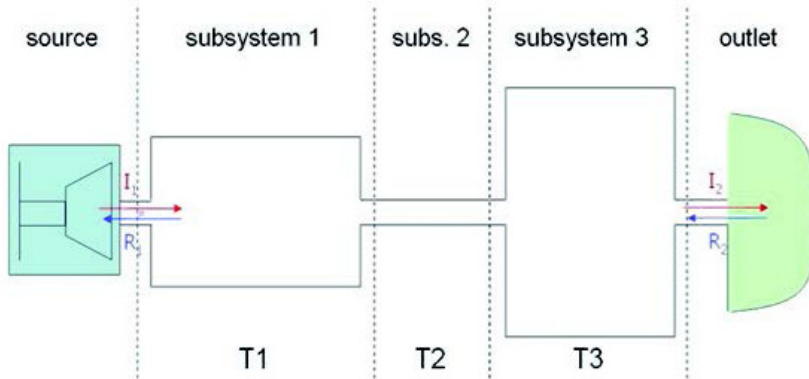
TMM (Transfer Matrix Method) for acoustic analysis of an entire exhaust line and its optimization
