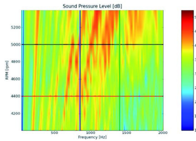
Waterfall diagram of the sound pressure level as a function of frequency and engine RPM
